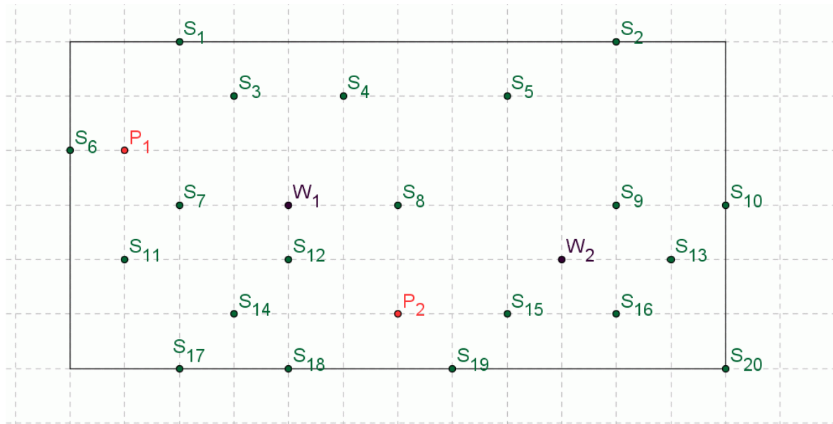
P = \text{plant}, W = \text{warehouse}, S = \text{shop}.
